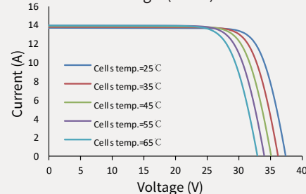
Current-Voltage (410W)
