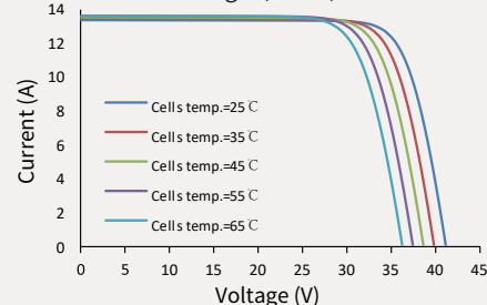
Current-Voltage (455W)
