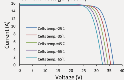
Current-Voltage (460W)
