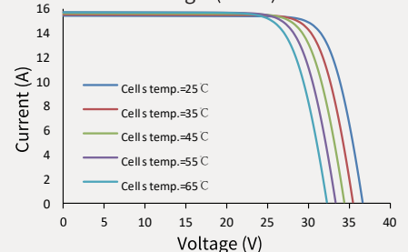
Current-Voltage (460W)
