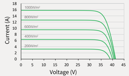
Power-Voltage (520W)
