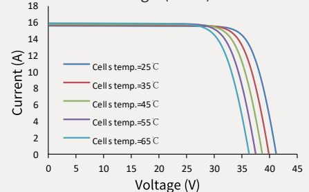
Current-Voltage (520W)
